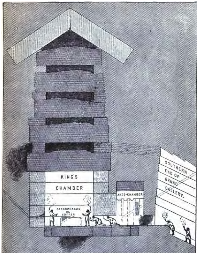
VERTICAL SECTION ( Looking West ) OF KING'S CHAMBER; ALSO OF ANTE-CHAMBER, SOUTH END OF GRAND GALLERY, AND VYSE'S HOLLOWAYS OF CONSTRUCTION, ABOVE KING'S CHAMBER, CROSSED LINES INDICATE GRANITE.
